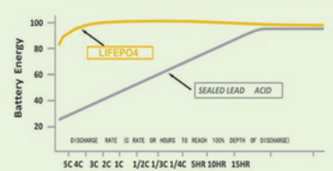
Energy Capacity VS. Discharge Rate
