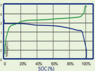
Charge / Discharge Curve SOC%
